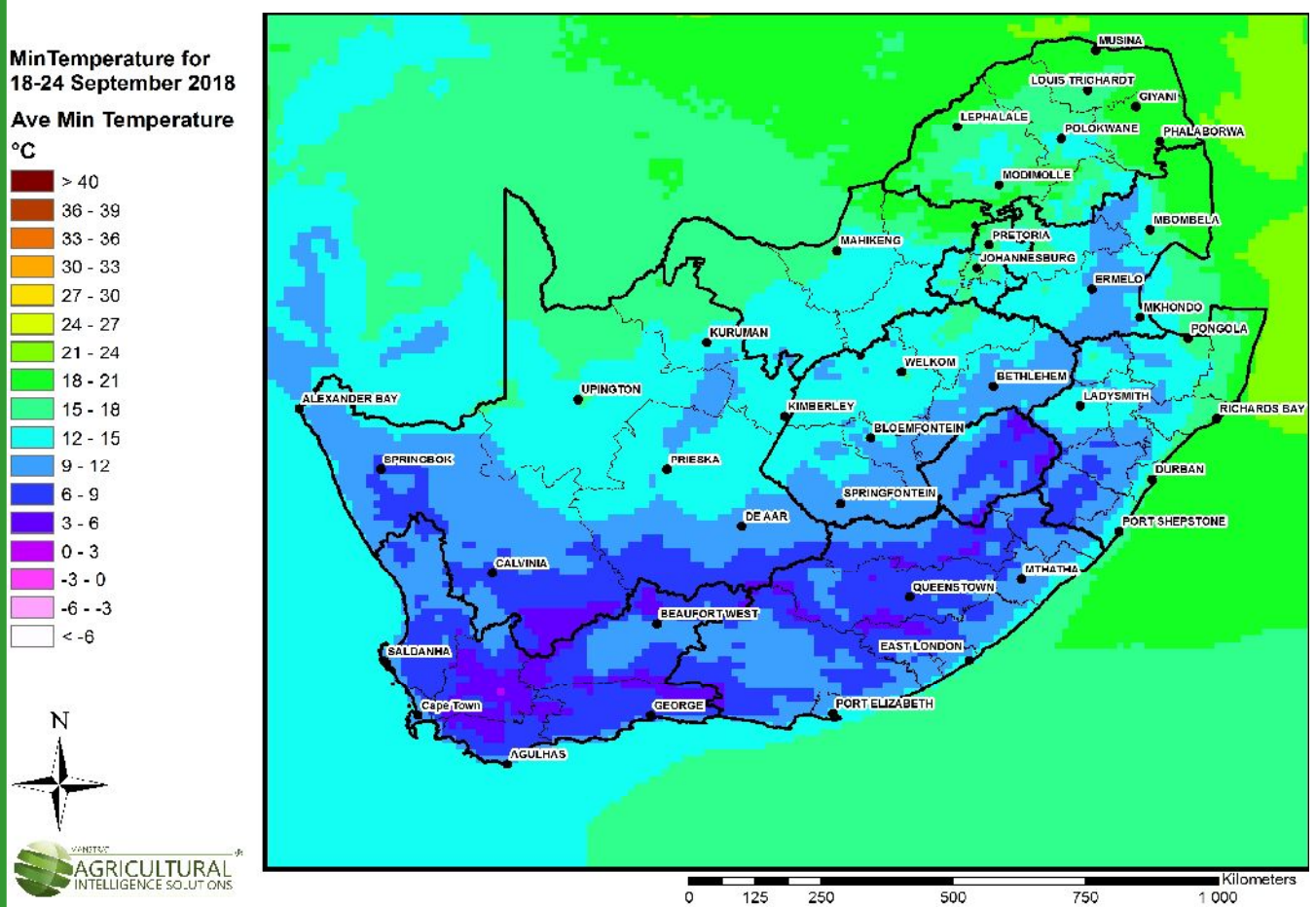
Figure 2: Average Minimum Temperatures: 18 to 24 September 2018.
