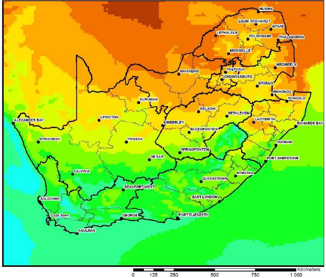
Figure 3: Average Maximum Temperatures: 18 to 24 September 2018.
