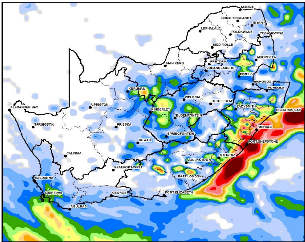
Figure 1: Expected precipitation 17 to 23 April 2018.
