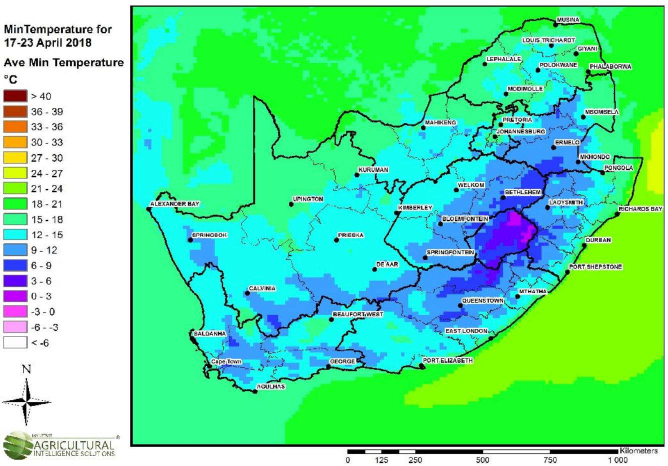
Figure 2: Average Minimum Temperatures 17 to 23 April 2018.
