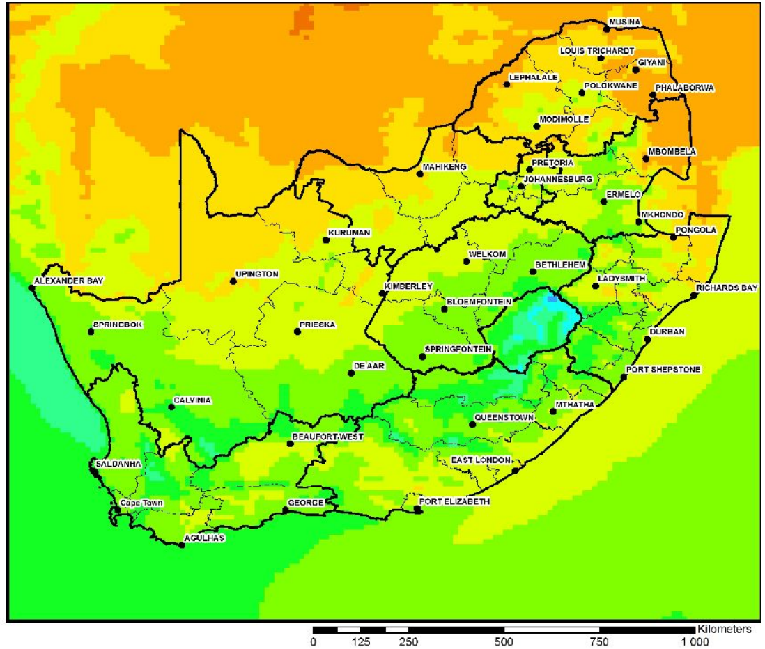
Figure 3: Average Maximum Temperatures 17 to 23 April 2018.
